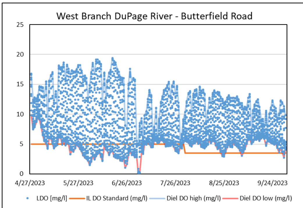
Figure 13. 2023 Dissolved Oxygen plot for the West Branch DuPage River at Butterfield Road (WBBR)
